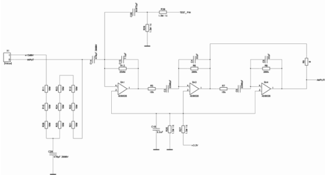
Figure 1 - Signal amplifier.
